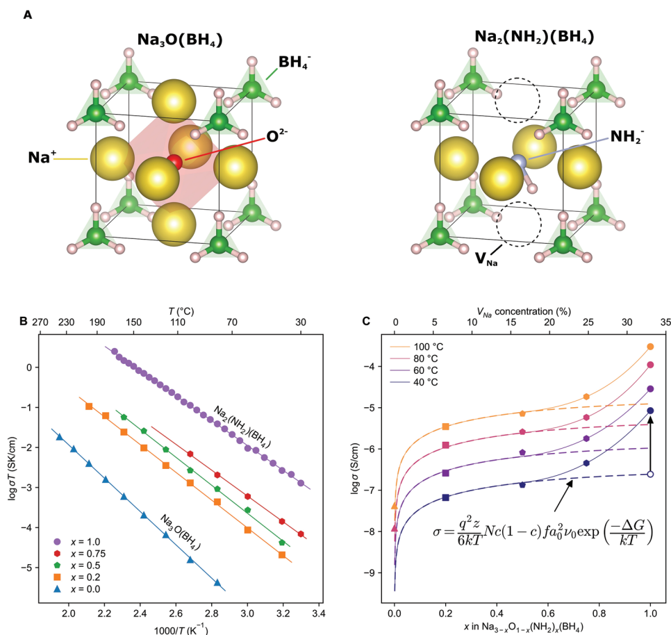
Figure 1. Sodium ion transport in \text{Na}_{3-x}\text{O}_{1-x}(\text{NH}_2)_x(\text{BH}_4) ( x = 0 - 1 ) upon systematic substitution of \text{O}^{2-} by \text{NH}_2^- , with corresponding increase in \text{Na}^+ vacancy concentration. A) Powder X-ray diffraction (PXRD) shows that the whole series of compositions \text{Na}_{3-x}\text{O}_{1-x}(\text{NH}_2)_x(\text{BH}_4) form cubic anti-perovskites with space group \text{Pm}\bar{3}\text{m} at room temperature (Figure S1, Supporting Information). Between the endmember compositions \text{Na}_3\text{O}(\text{BH}_4) and \text{Na}_2(\text{NH}_2)(\text{BH}_4) , the \text{Na}^+ vacancy concentration increases from zero to one-third at the full substitution of \text{O}^{2-} by \text{NH}_2^- . In the cubic unit cell \text{Na}_3\text{O}(\text{BH}_4) (A, left), \text{Na}^+ ions at the face-centered sites comprise the vertices of the \text{Na}_6\text{O} octahedra, and (\text{BH}_4)^- cluster anions occupy the corner sites. In the cubic unit cell \text{Na}_2(\text{NH}_2)(\text{BH}_4) (A, right), two of the six \text{Na}^+ ions are missing, and the \text{O}^{2-} ion residing at the center of the pseudo-octahedron is replaced with an \text{NH}_2^- anion. B) Temperature-dependent ionic conductivity of \text{Na}_{3-x}\text{O}_{1-x}(\text{NH}_2)_x(\text{BH}_4) (where x = 0, 0.2, 0.5, 0.75 , and 1.0 ) exhibits Arrhenius behavior above the room temperature region and ionic conductivity increases with the substitution of \text{O}^{2-} by \text{NH}_2^- . Activation energies are 0.358, 0.299, 0.301, 0.278, and 0.268 eV respectively. The endmember composition \text{Na}_2(\text{NH}_2)(\text{BH}_4) with the highest \text{Na}^+ vacancy and \text{NH}_2^- cluster anion concentration shows 10^4 higher ionic conductivity than that of the endmember \text{Na}_3\text{O}(\text{BH}_4) without the substitution of \text{NH}_2^- . C) The dependence of ionic conductivity on the concentration of \text{Na}^+ vacancy and \text{NH}_2^- cluster ion concentration at several temperatures between 40 °C and 100 °C is fitted as the dashed line using the vacancy-dependent ionic conductivity model (inset equation). At low x ( \leq 0.75 ), the ionic conductivity can be fit well by the classical vacancy-concentration model. At high x ( > 0.75 ), ionic conductivity of \text{Na}_{3-x}\text{O}_{1-x}(\text{NH}_2)_x(\text{BH}_4) exhibits a large positive deviation from the expected classical vacancy-dependent conductivity. It is correlated with not only high vacancy concentration but also the \text{NH}_2^- cluster anion concentration, suggesting a paddle-wheel effect.
