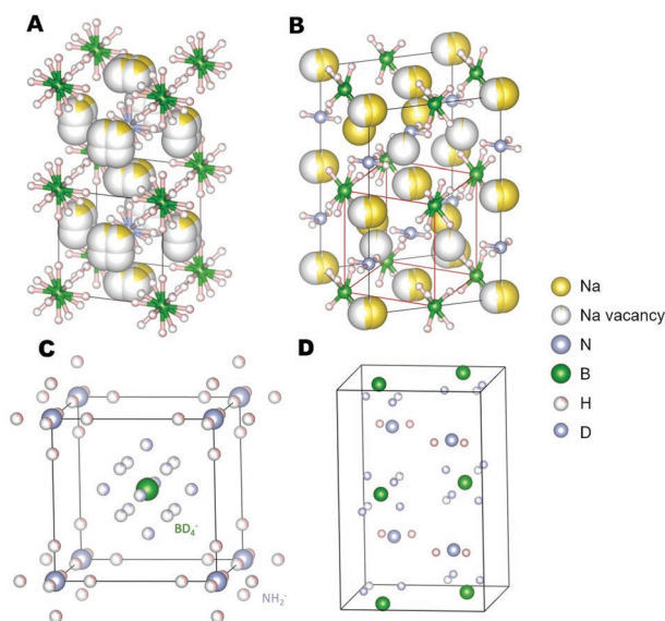
Figure 2. A) Two vertically stacked \text{Na}_2(\text{NH}_2)(\text{BH}_4) cubic unit cells and B) one orthorhombic unit cell with corresponding cubic unit cell marked with red lines, from Rietveld refinement of synchrotron XRD data. The cubic phase exhibits greater vacancy and anion rotational disorder compared to the orthorhombic phase. C) \text{Na}_2(\text{NH}_2)(^{11}\text{BD}_4) cubic unit cell and D) orthorhombic unit cells from Rietveld refinement of neutron diffraction data with sodium removed for clarity. Neutron diffraction is more sensitive to the light hydrogen and deuterium and confirms the increased ordering of anion orientation in the orthorhombic phase.
