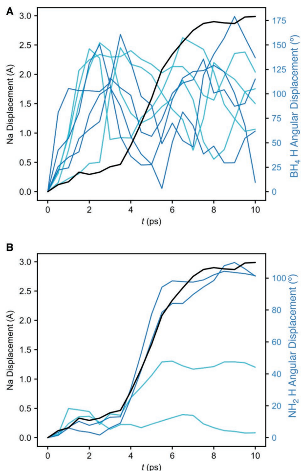
Figure 4. Correlation between sodium ion translation (left vertical axis, black line) and cluster anion angular displacement (right vertical axis, blue lines, the shade is indicative of which of the two nearest neighbors the hydrogen belongs to) plotted against time during a representative migration event in a 50 ps AIMD simulation of \text{Na}_2(\text{NH}_2)(\text{BH}_4) at 363 K (for additional migration events see Figure S9 in the Supporting Information). A) Borohydride rotation is faster but less synchronized with sodium migration, while B) amide rotation is slower but highly synchronized.
