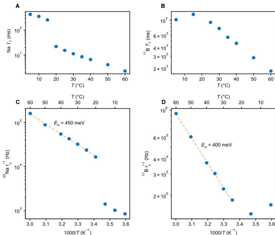
Figure 5. Experimental A) ^{23}\text{Na} and B) ^{11}\text{B} T_1 relaxation times of \text{Na}_2(\text{NH}_2)(\text{BH}_4) measured as a function of temperature; the phase transition is apparent as the sudden increase in ^{23}\text{Na} T_1 . C,D) Correlation times \tau_c extracted from the T_1 values in (A) and (B) respectively, using the following equation derived from the BPP theory:
